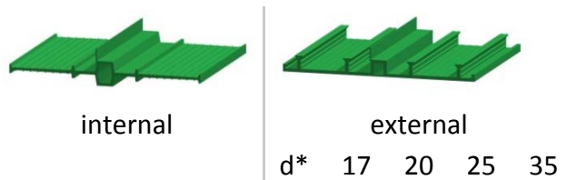
Expansion joint tape
